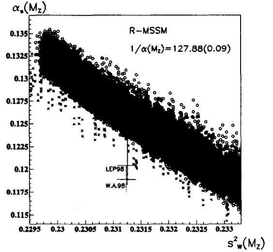
Figure 3. \alpha_s(M_Z) versus \hat{s}_Z for the MSSM (circles) and for the bilinear R_p model (crosses).
