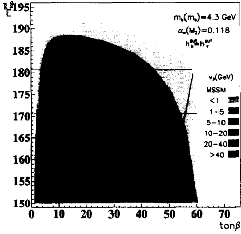
Figure 2. Top quark mass as a function of \tan \beta for different values of the R-Parity violating parameter v_3 .
