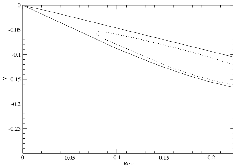
Figure 3: In the case m_3 > m_{1,2} , the region in the \nu - \text{Re } \epsilon plane inside the full line is excluded by (5.13) when \text{Im } \epsilon = 10^{-4} . The region inside the dotted line is excluded when \text{Im } \epsilon = 5 \times 10^{-3} . For \text{Im } \epsilon larger than 10^{-2} there is no excluded region any more.
