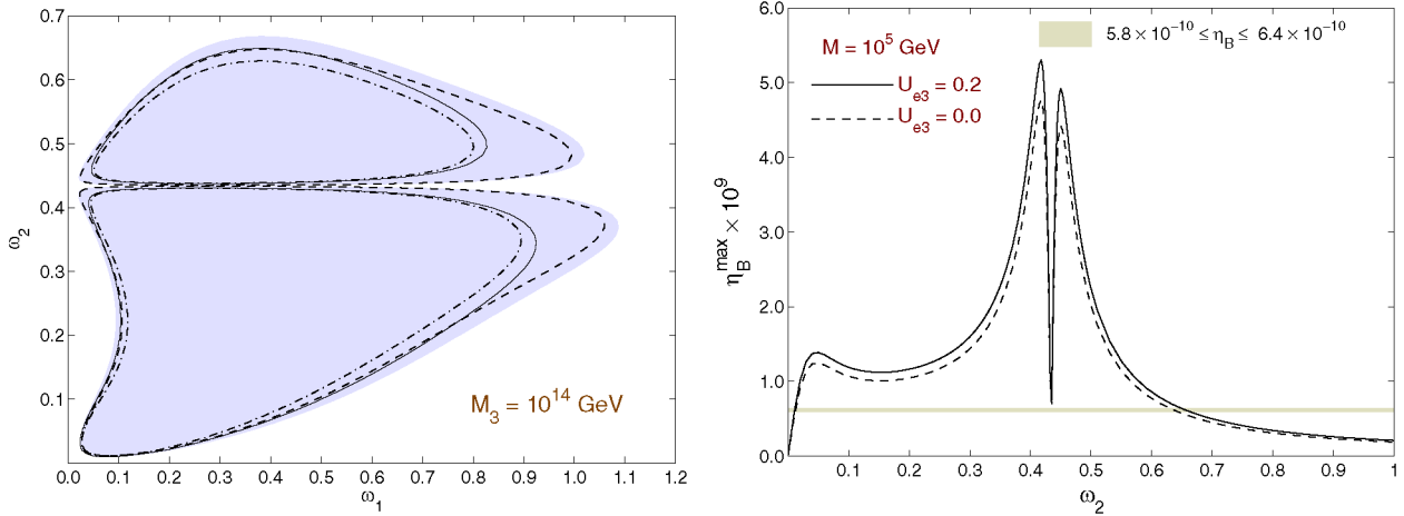
Fig. 2. The baryon asymmetry as a function of \omega_1 and \omega_2 in the case m_1 = 0, \theta_3 = 0 for U_{e3} = 0, 0.2 ; M = 10^5, 10^{10} GeV and M_3 = 10^{14} GeV. The line and colour schemes are the same as used in Fig. 1. On the left plot, the region in the (\omega_1, \omega_2) -plane where the value of \eta_B \geq 5.8 \times 10^{-10} is shown. The maximal value of \eta_B as a function of \omega_2 is shown in the right plot for the same values of U_{e3} and M = 10^5 GeV.
